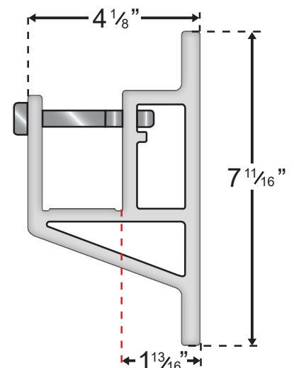
Wall and Soffit Bracket - Side View
