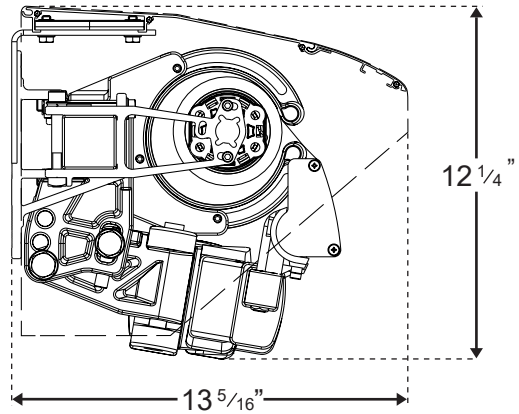
SUMMIT - Wall Mount (with hood)
