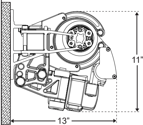
SUMMIT - Wall Mount (without hood)
