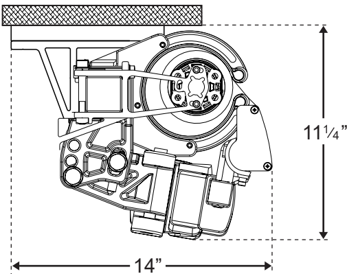
SUMMIT - Soffit Mount (no hood option available)
