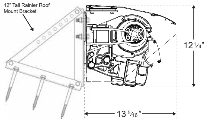
SUMMIT - Roof Mount (with 12" roof brackets & hood)
